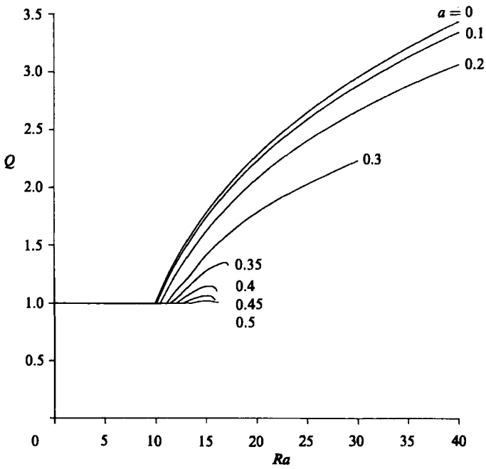
FIGURE 15. The Nusselt number based on the heat transfer at Ra = 0 for type-II flows.
