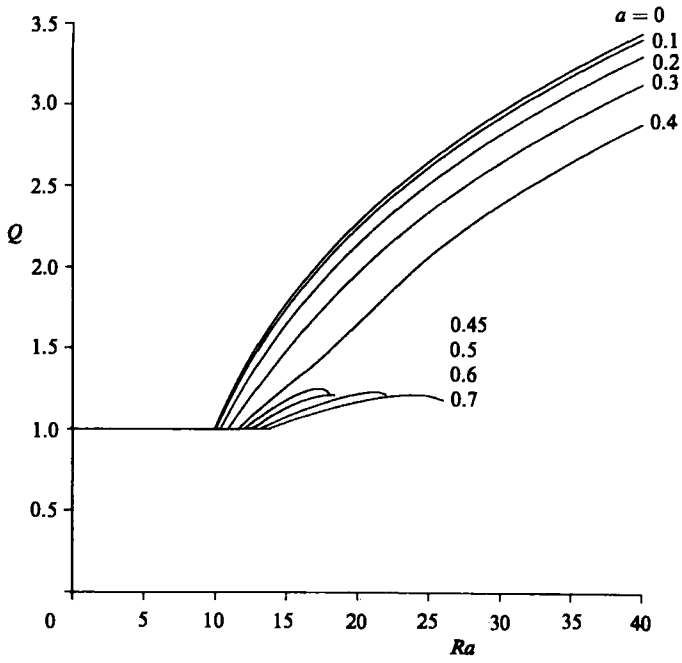
FIGURE 14. The Nusselt number based on the heat transfer at Ra = 0 for type-I flows.
