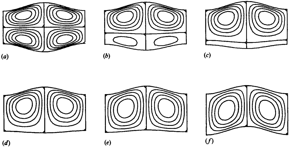
FIGURE 2. The O(\delta) streamlines as calculated from equation (3.12a) for Ra = 5 , \beta = 0 and wall amplitudes (a) a_1 = a_u , (b) a_1 = 0.75a_u , (c) a_1 = 0.5a_u , (d) a_1 = 0.25a_u , (e) a_1 = -0.25a_u , (f) a_1 = -a_u .
