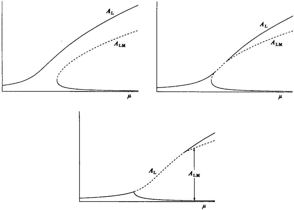
FIGURE 6. An illustration of the three possible regimes for the stability and existence of longitudinal and mixed modes for the general undulating layer: —, stable solutions; -----, unstable solutions.
