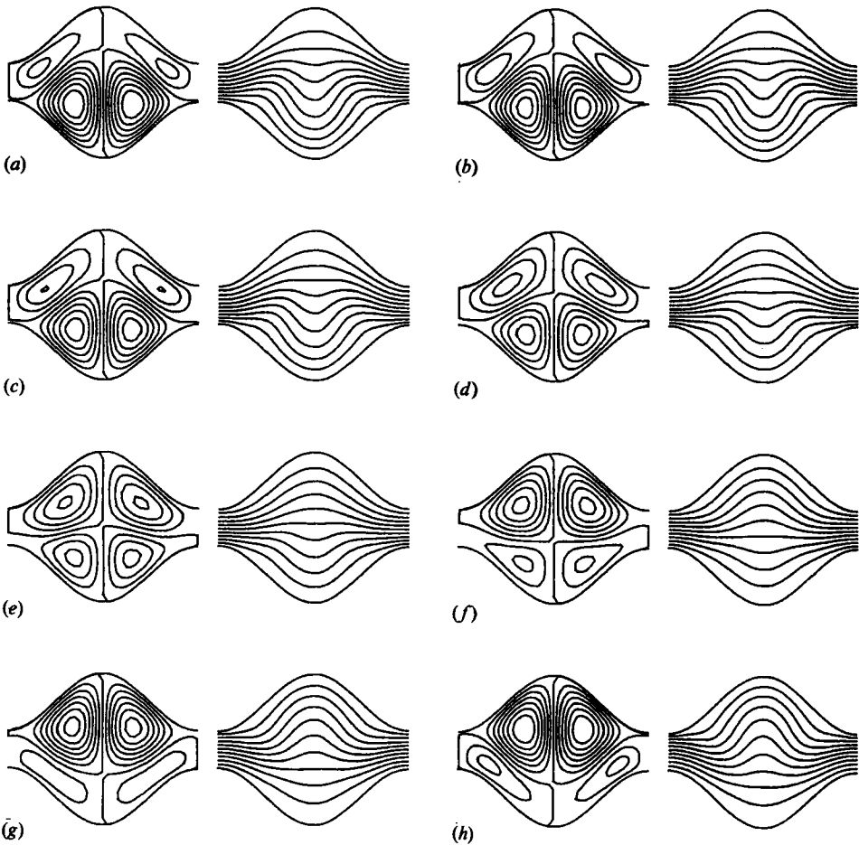
FIGURE 19. Instantaneous streamlines and isotherms for Ra = 19 , \alpha = 0.6 , type II, for half a cycle. (a) corresponds to the maximum of \psi_{\max} , and consecutive plots are at equal time increments.
